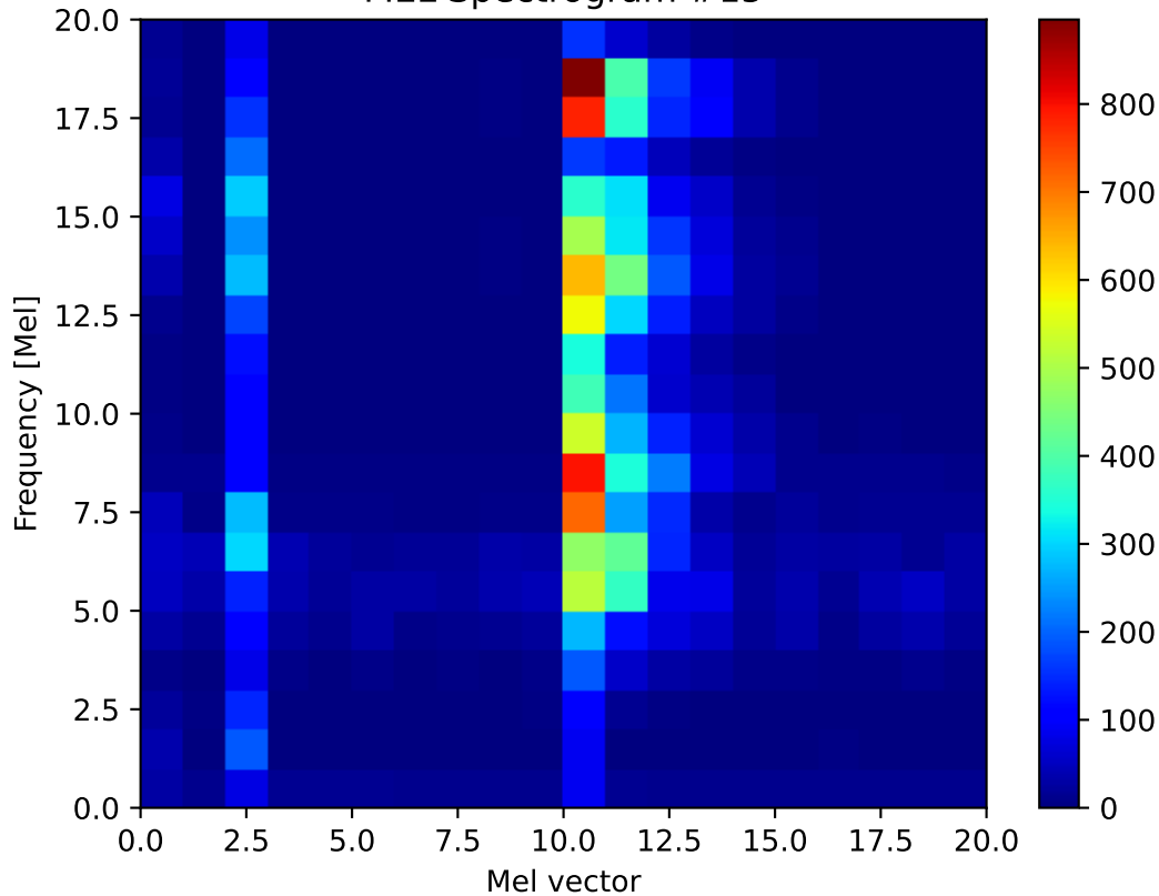
MEL Spectrogram #15
